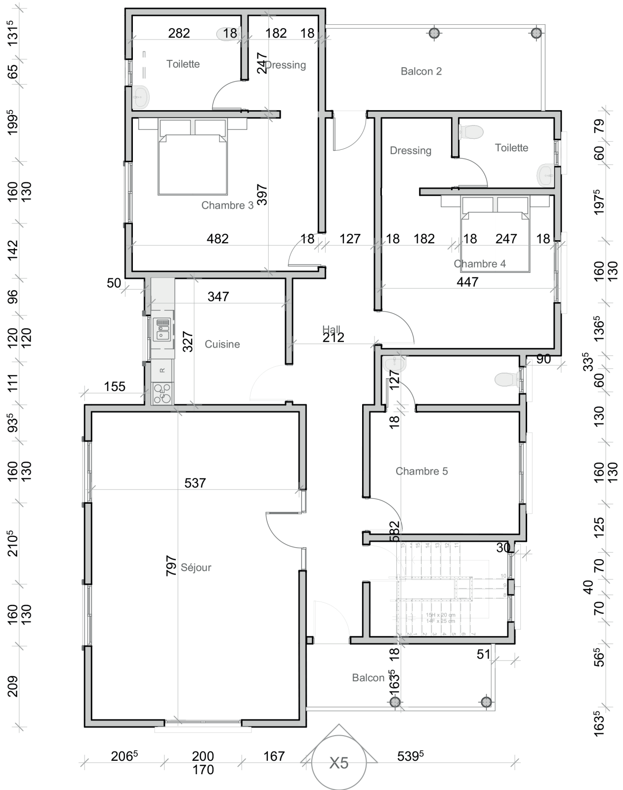
PLAN TYPE R+1
