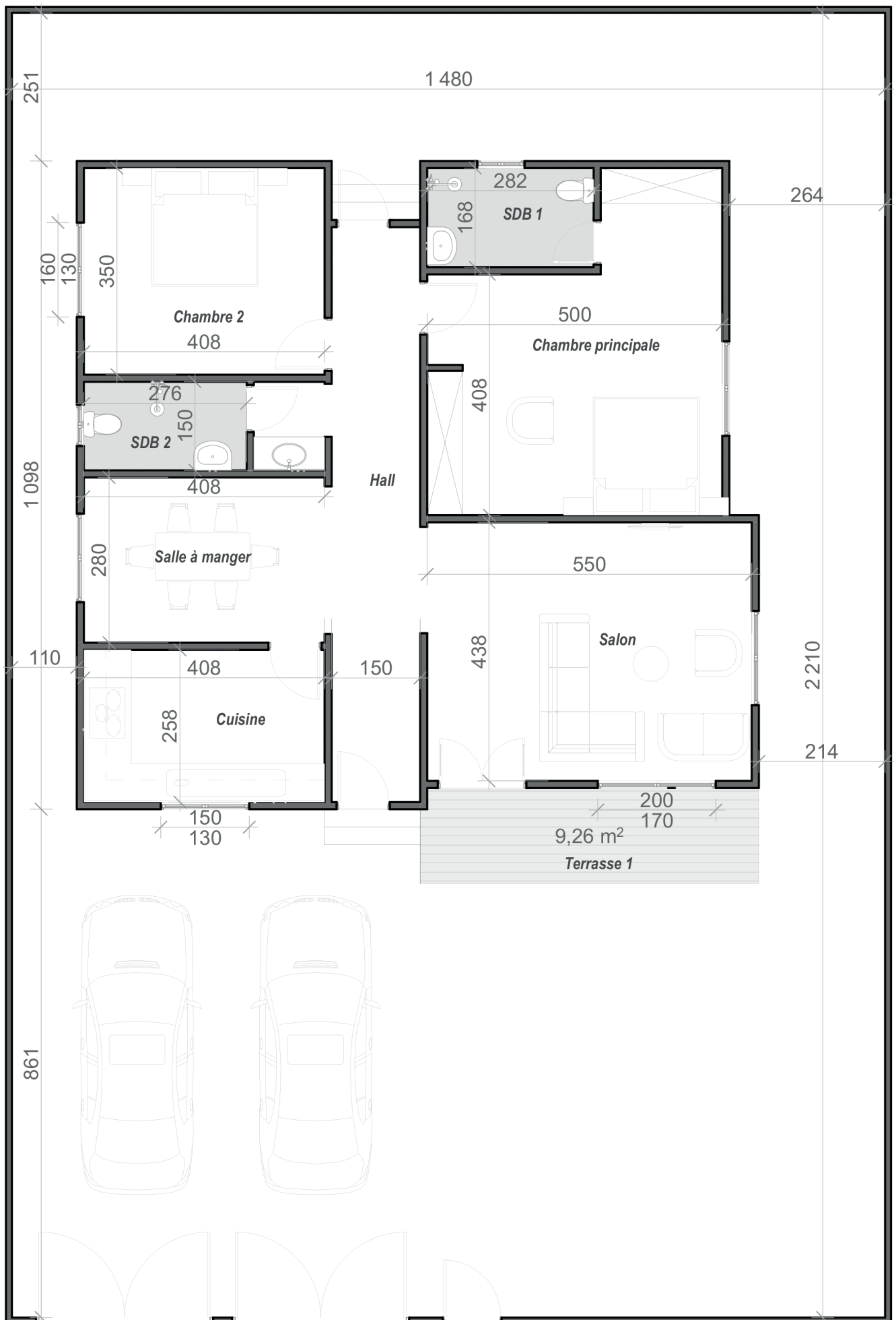
PLAN TYPE F3 DRABO
